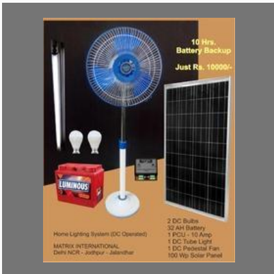
Solar DC Operated Home Lighting System
